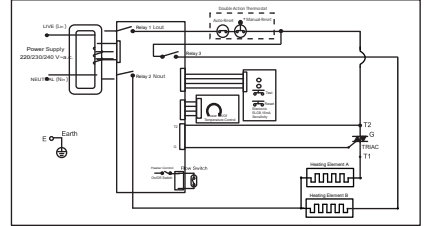
WIRING DIAGRAM -WITH ELCB, NO PUMP DPDT MODEL (FOR VIETNAM MODELS ONLY)
